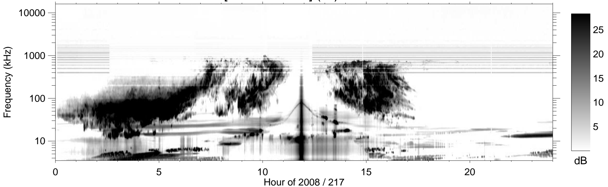
RPWS [ABCH1H2/Ex] (-B) 2008/08/04
