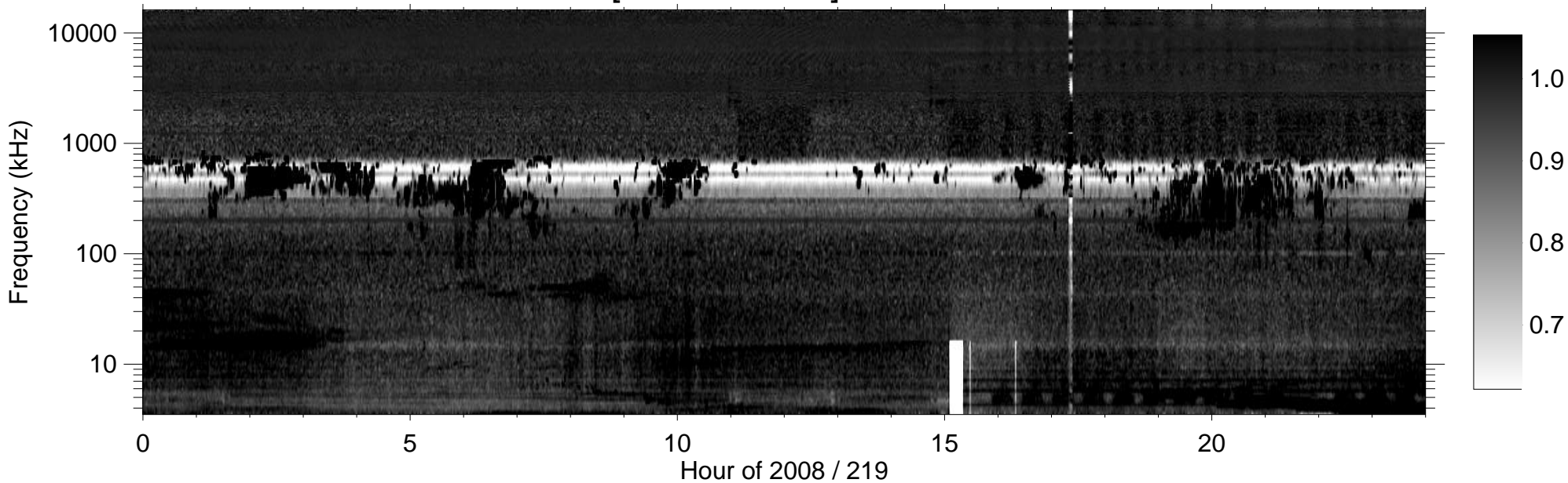
RPWS [ABCH1H2/Ex] (-B) 2008/08/06
