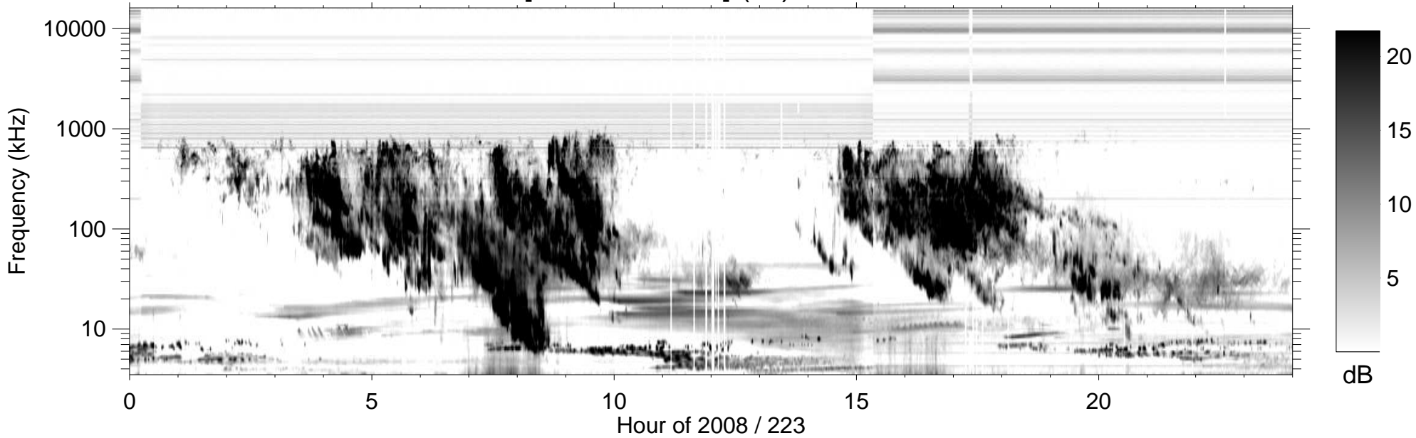
RPWS [ABCH1H2/Ex] (-B) 2008/08/10
