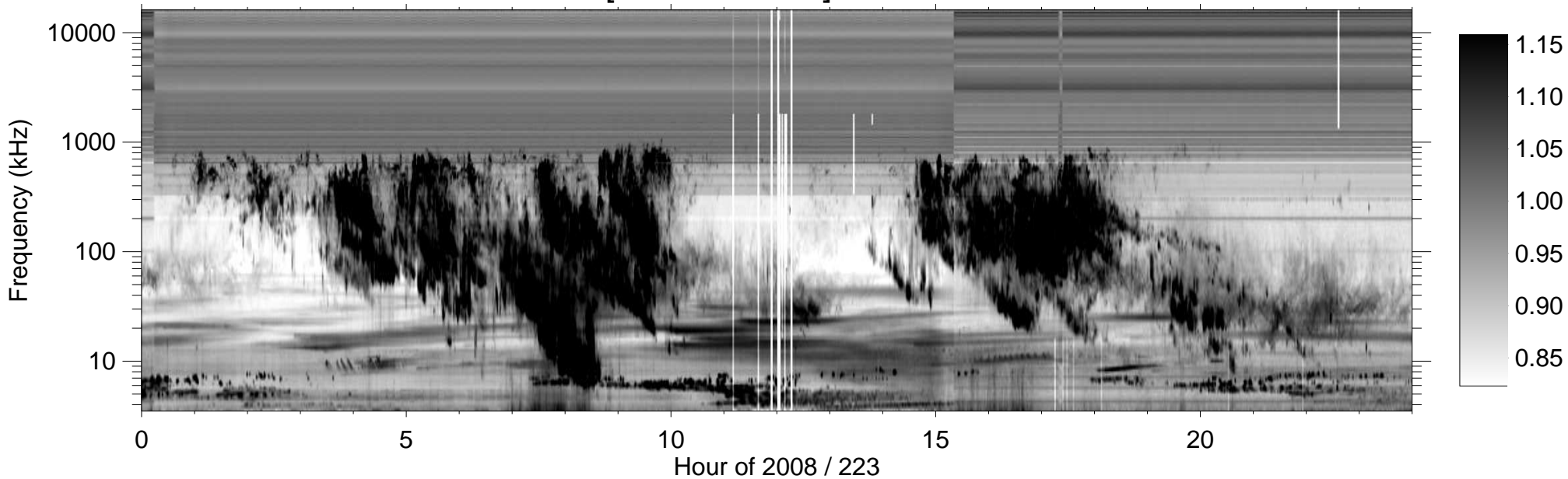
RPWS [ABCH1H2/Ex] (-B) 2008/08/10
