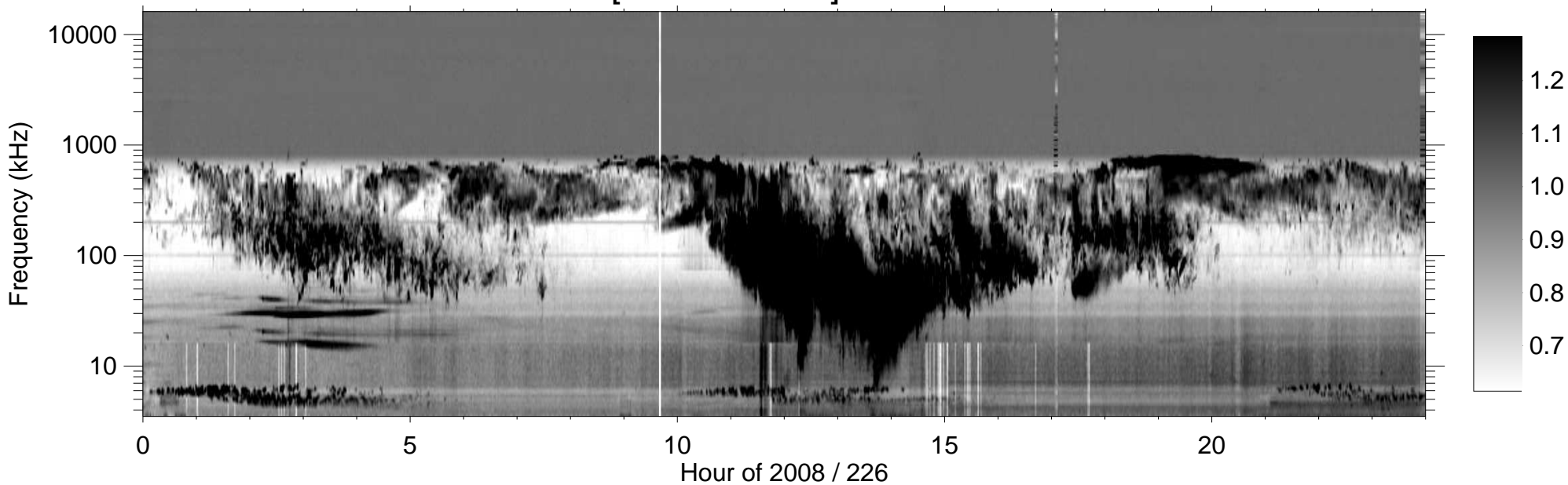
RPWS [ABCH1H2/Ex] (-B) 2008/08/13
