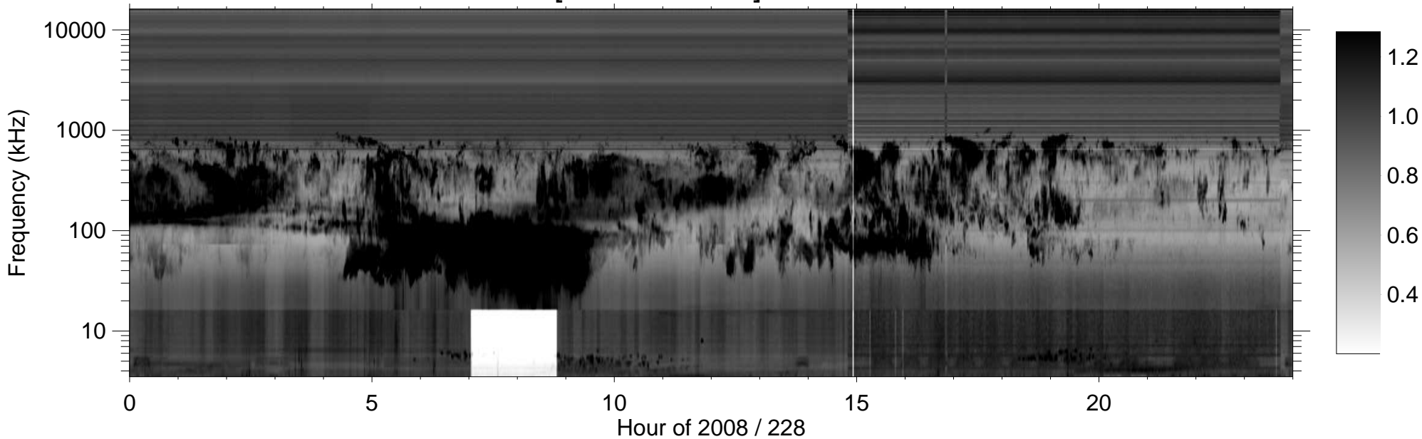
RPWS [ABCH1H2/Ex] (-B) 2008/08/15
