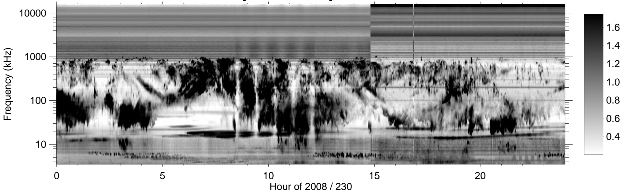
RPWS [ABCH1H2/Ex] (-B) 2008/08/17
