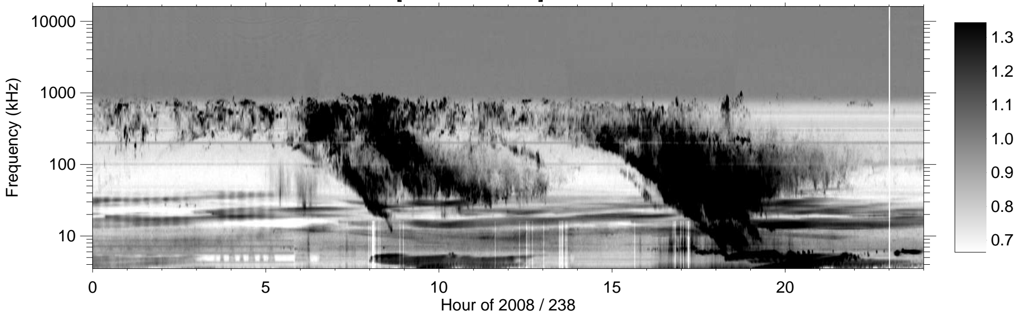
RPWS [ABCH1H2/Ex] (-B) 2008/08/25
