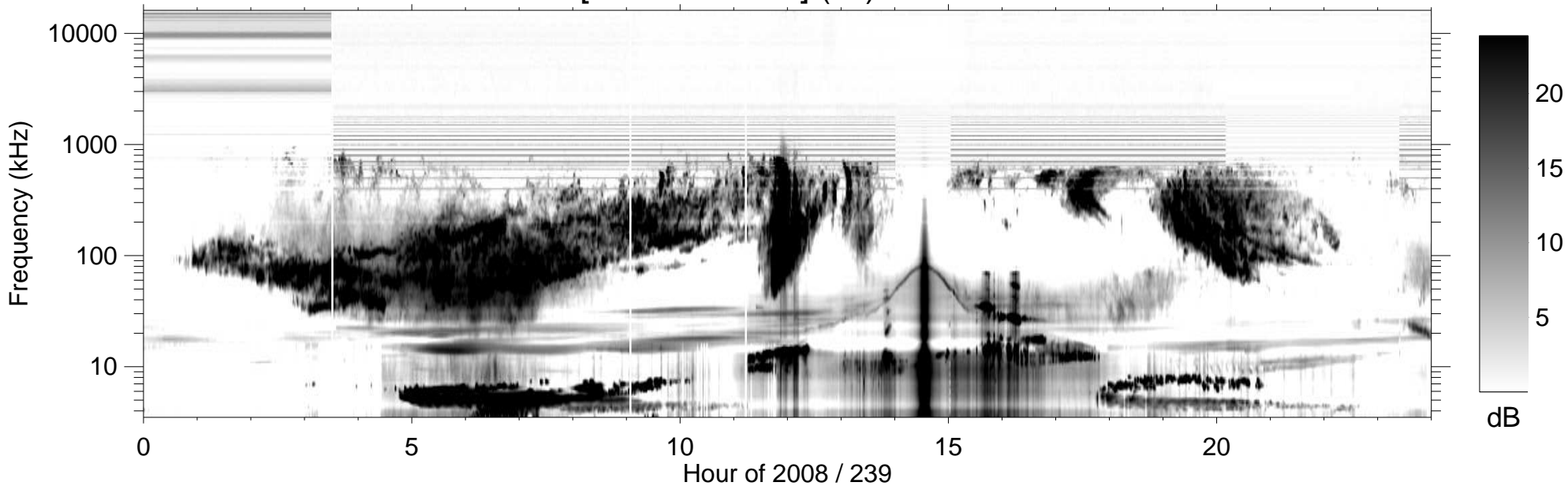
RPWS [ABCH1H2/Ex] (-B) 2008/08/26
