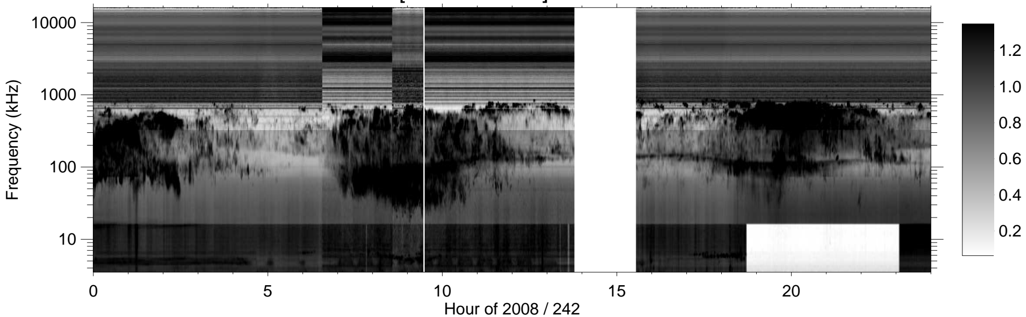
RPWS [ABCH1H2/Ex] (-B) 2008/08/29
