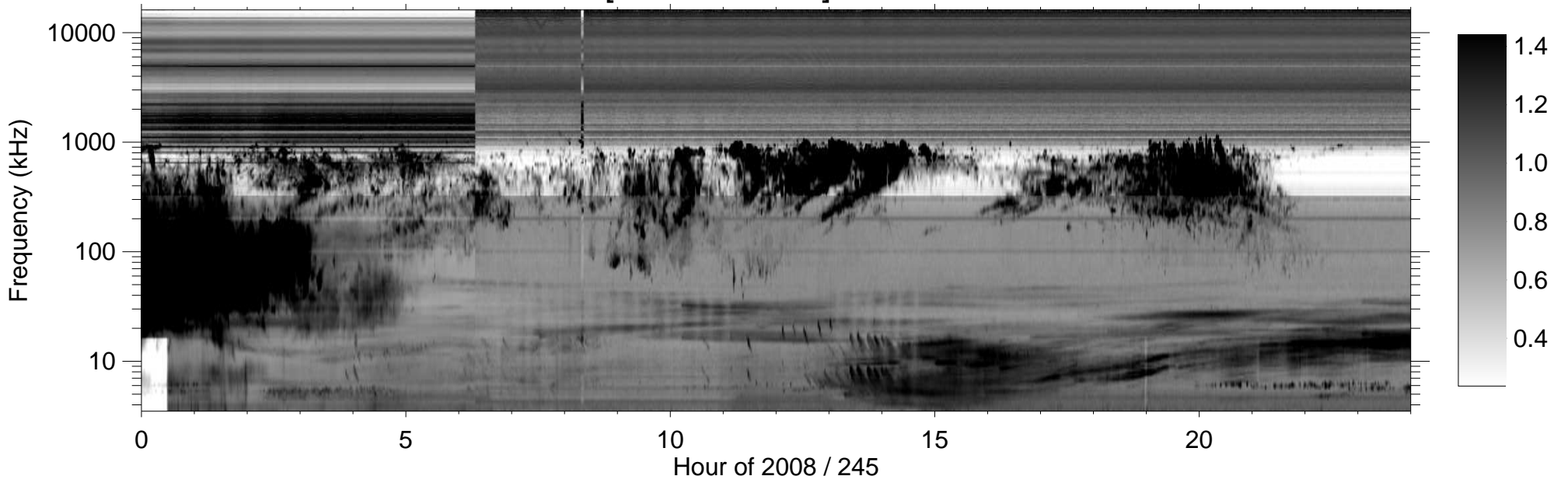
RPWS [ABCH1H2/Ex] (-B) 2008/09/01
