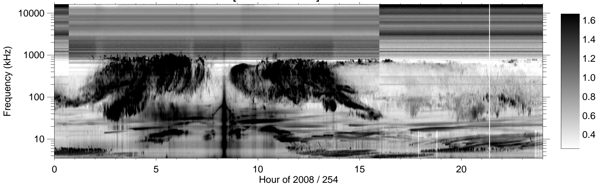
RPWS [ABCH1H2/Ex] (-B) 2008/09/10
