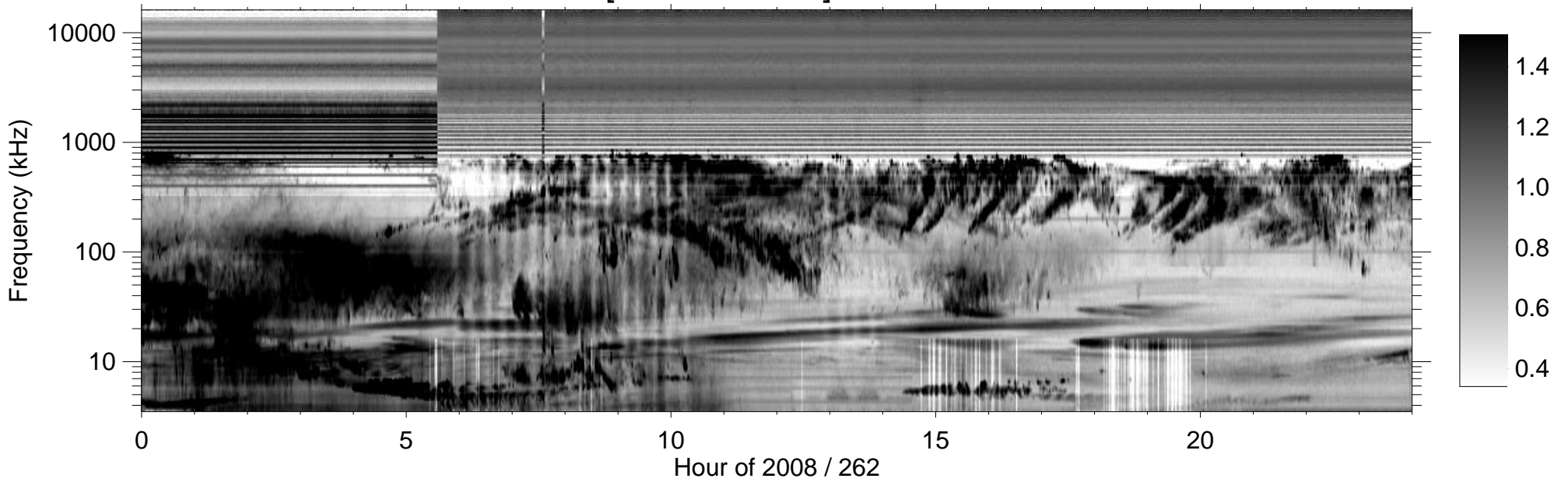
RPWS [ABCH1H2/Ex] (-B) 2008/09/18
