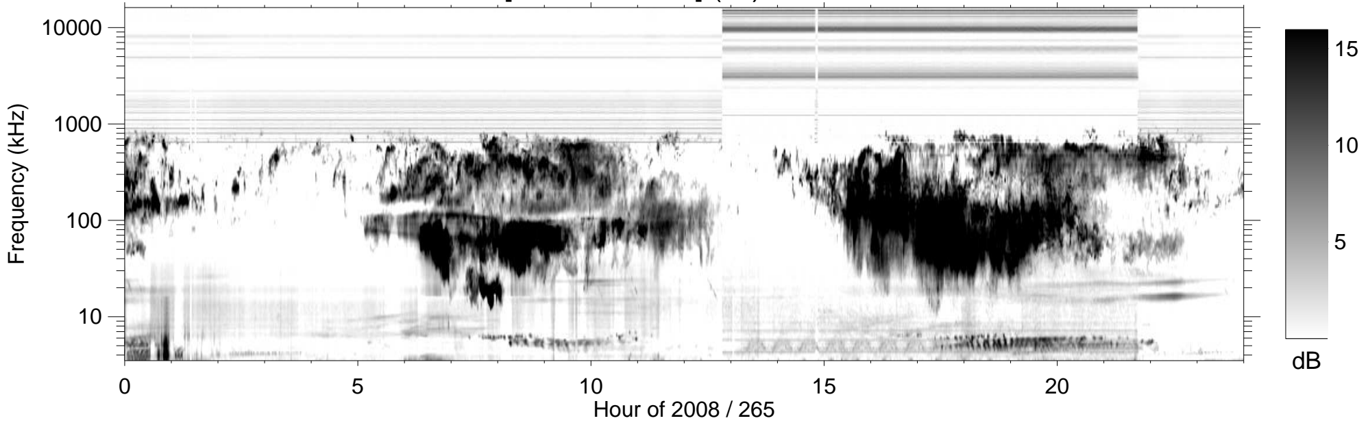
RPWS [ABCH1H2/Ex] (-B) 2008/09/21
