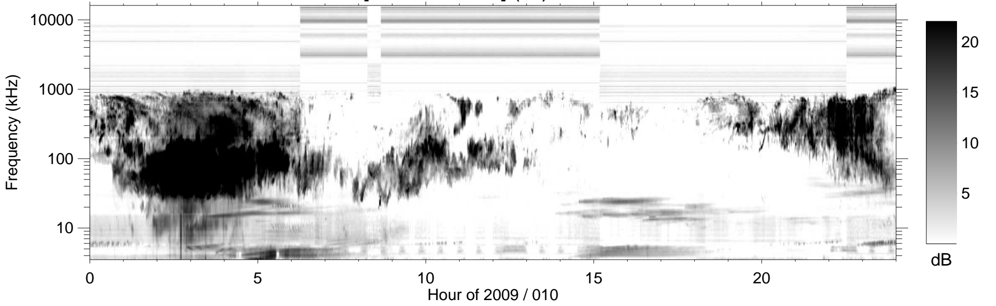
RPWS [ABCH1H2/Ex] (-B) 2009/01/10
