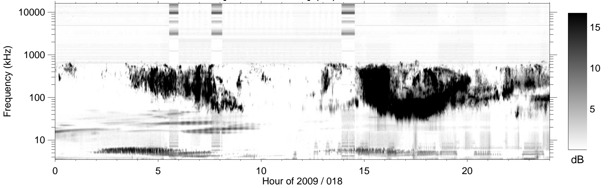
RPWS [ABCH1H2/Ex] (-B) 2009/01/18
