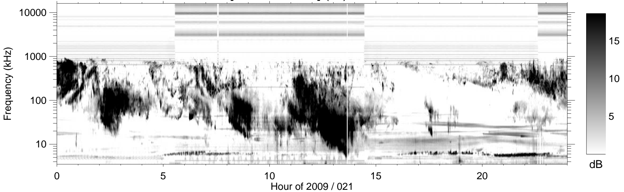
RPWS [ABCH1H2/Ex] (-B) 2009/01/21
