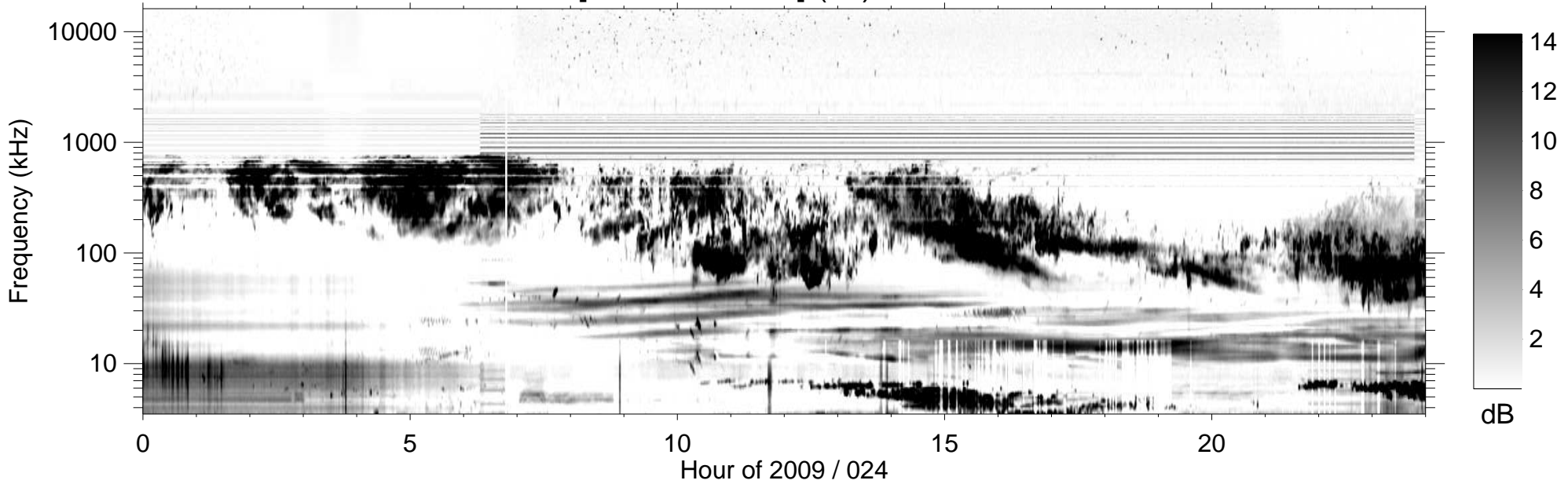
RPWS [ABCH1H2/Ex] (-B) 2009/01/24
