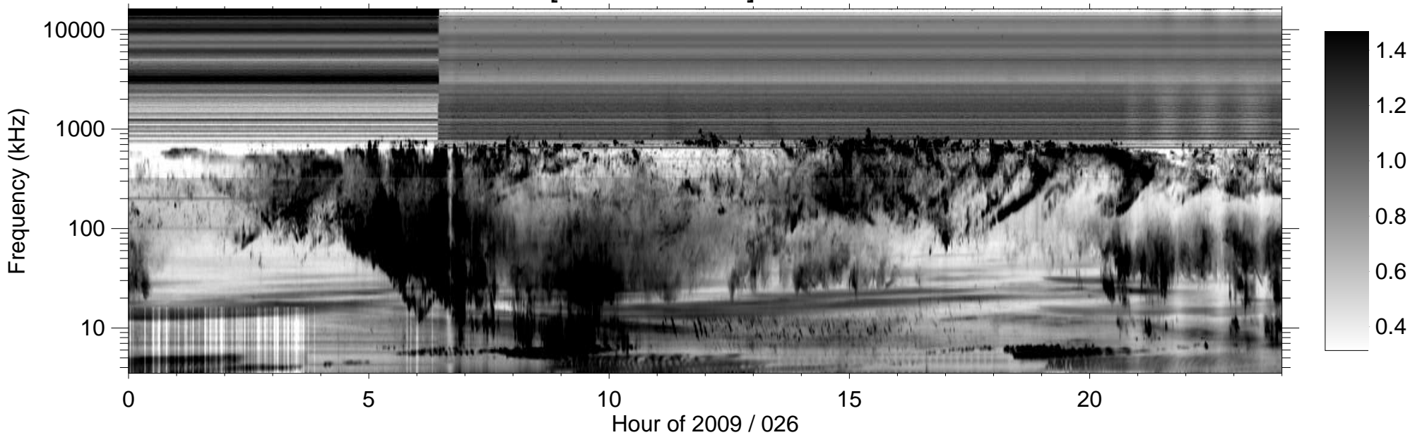
RPWS [ABCH1H2/Ex] (-B) 2009/01/26
