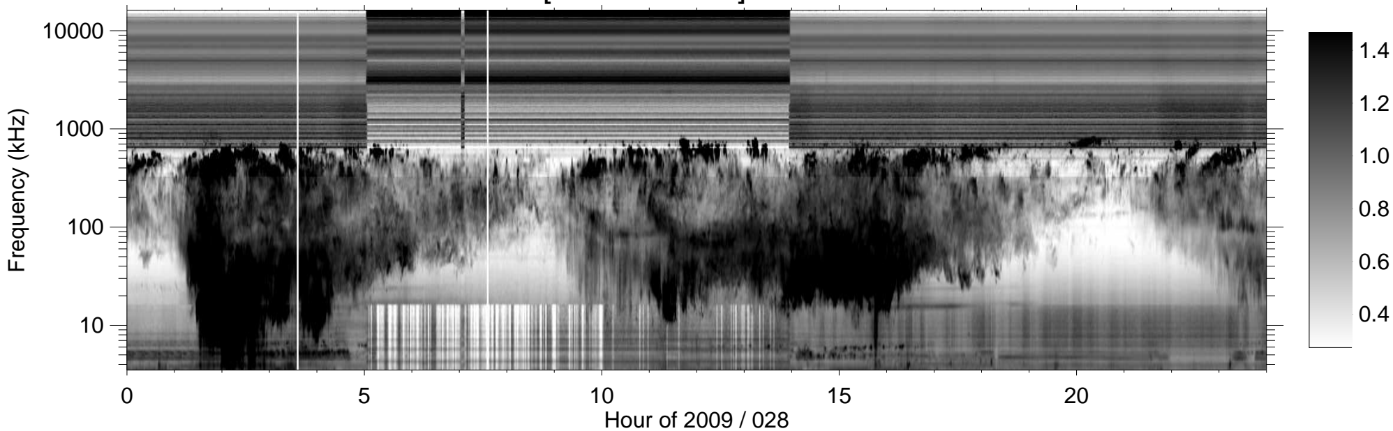
RPWS [ABCH1H2/Ex] (-B) 2009/01/28
