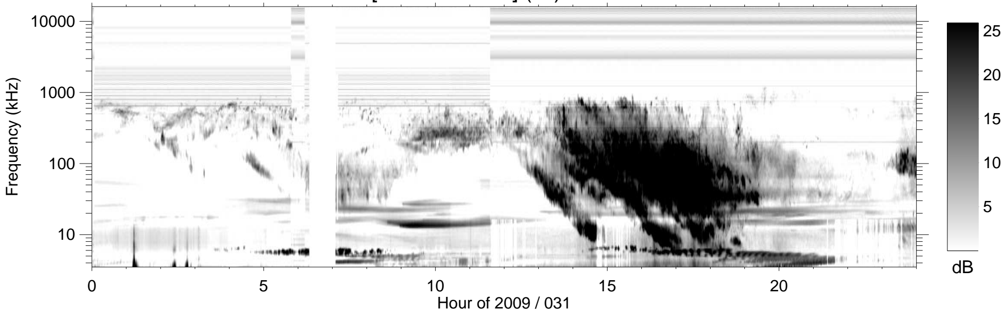
RPWS [ABCH1H2/Ex] (-B) 2009/01/31
