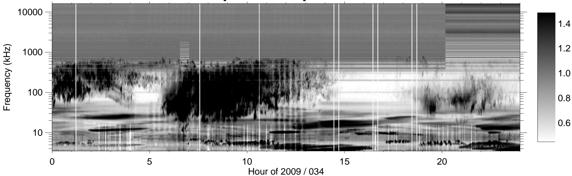
RPWS [ABCH1H2/Ex] (-B) 2009/02/03
