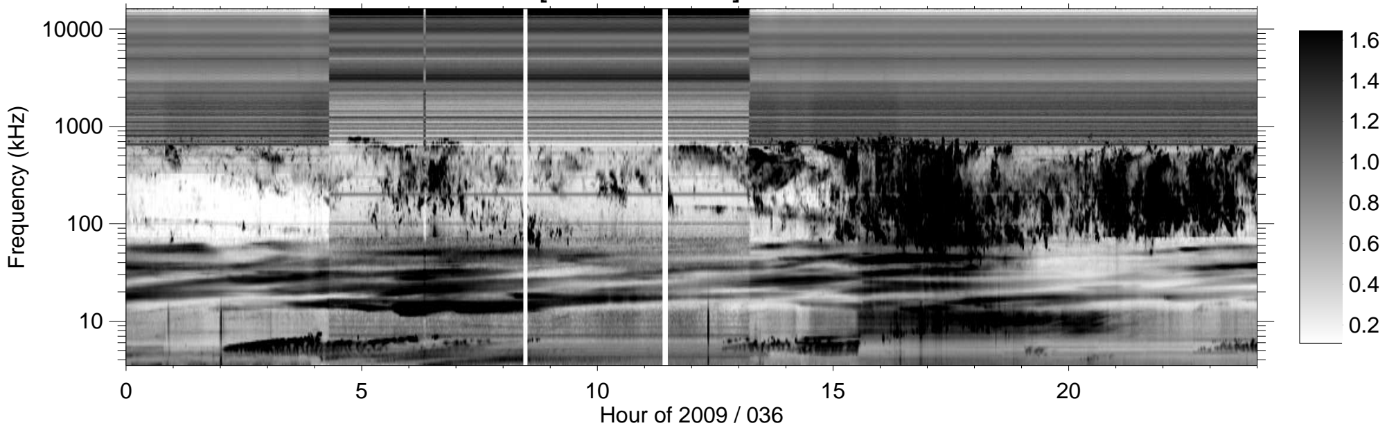
RPWS [ABCH1H2/Ex] (-B) 2009/02/05
