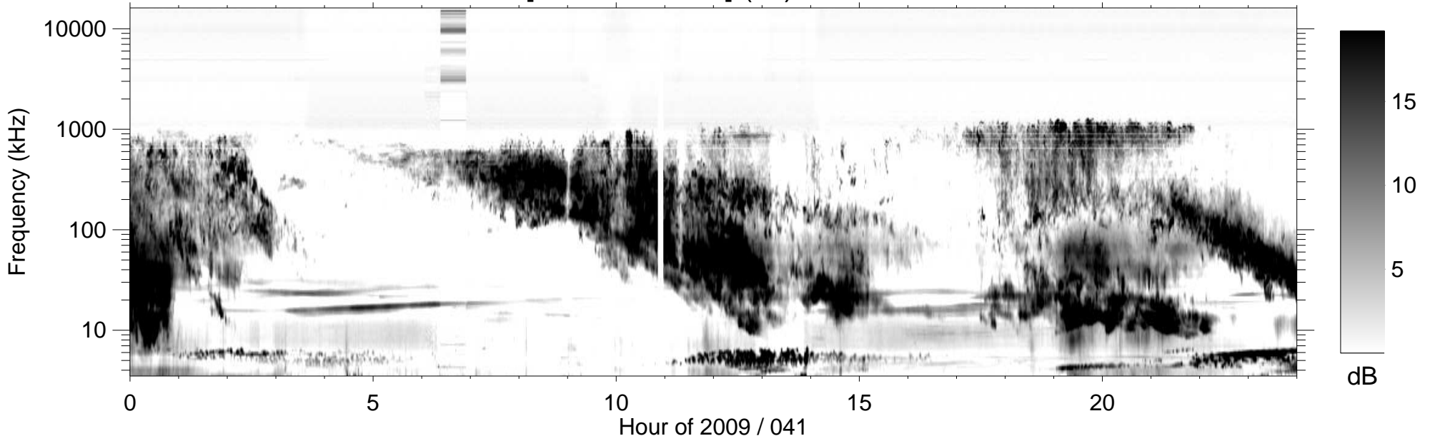
RPWS [ABCH1H2/Ex] (-B) 2009/02/10
