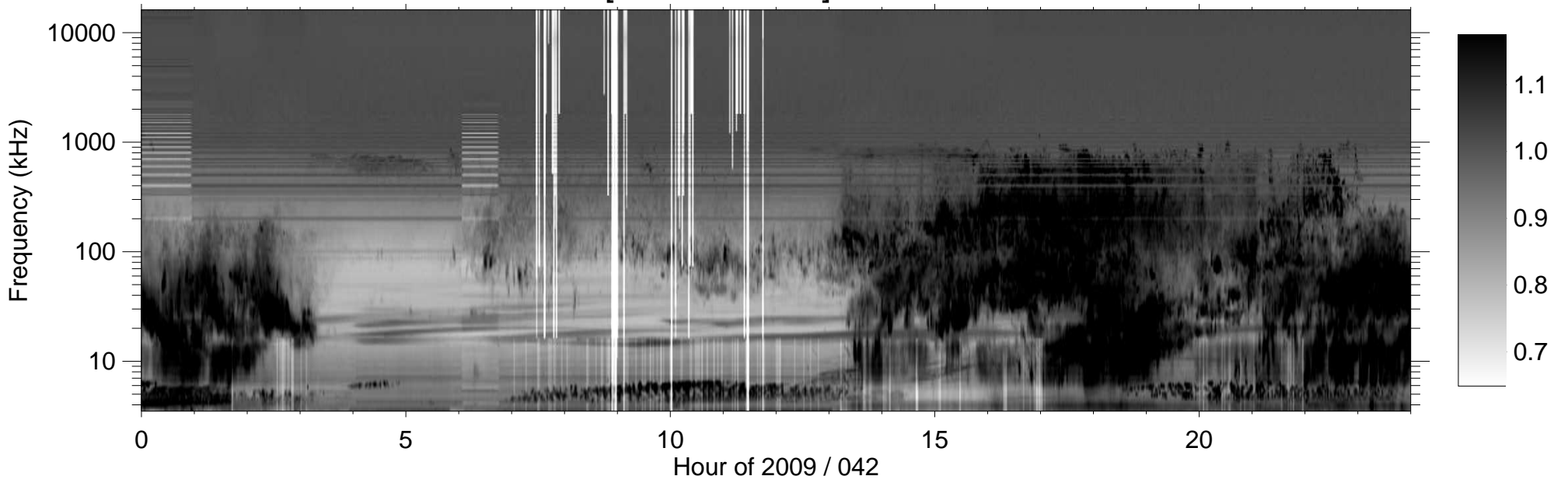
RPWS [ABCH1H2/Ex] (-B) 2009/02/11
