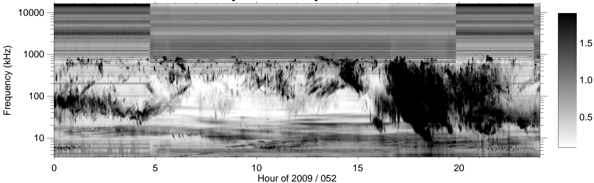
RPWS [ABCH1H2/Ex] (-B) 2009/02/21
