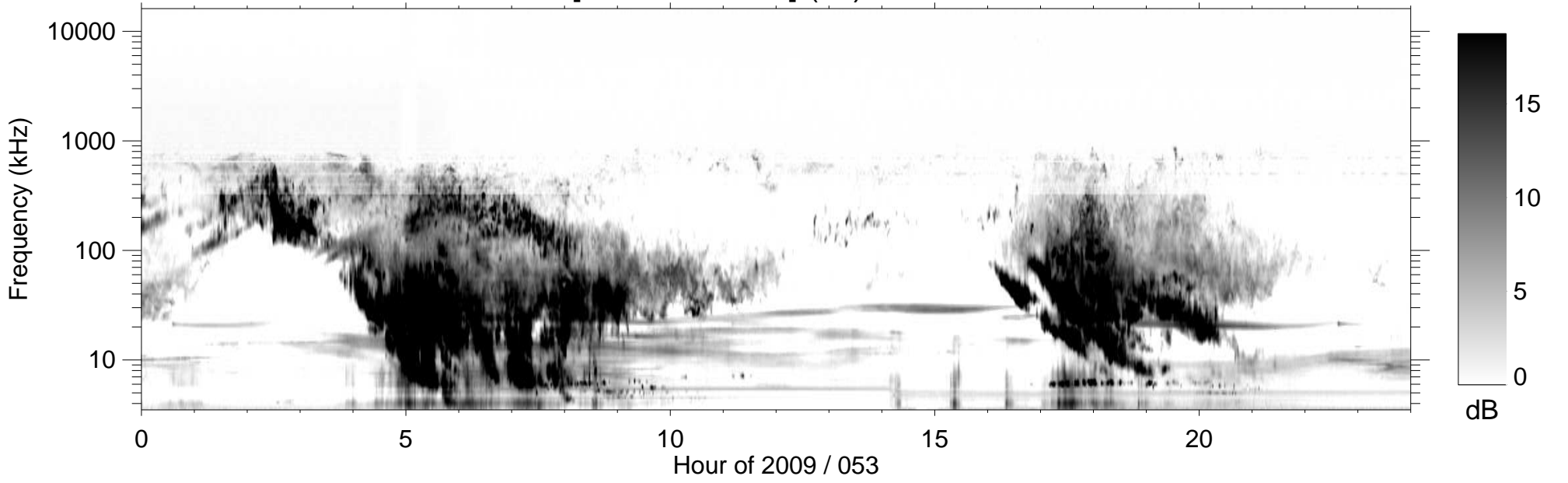
RPWS [ABCH1H2/Ex] (-B) 2009/02/22
