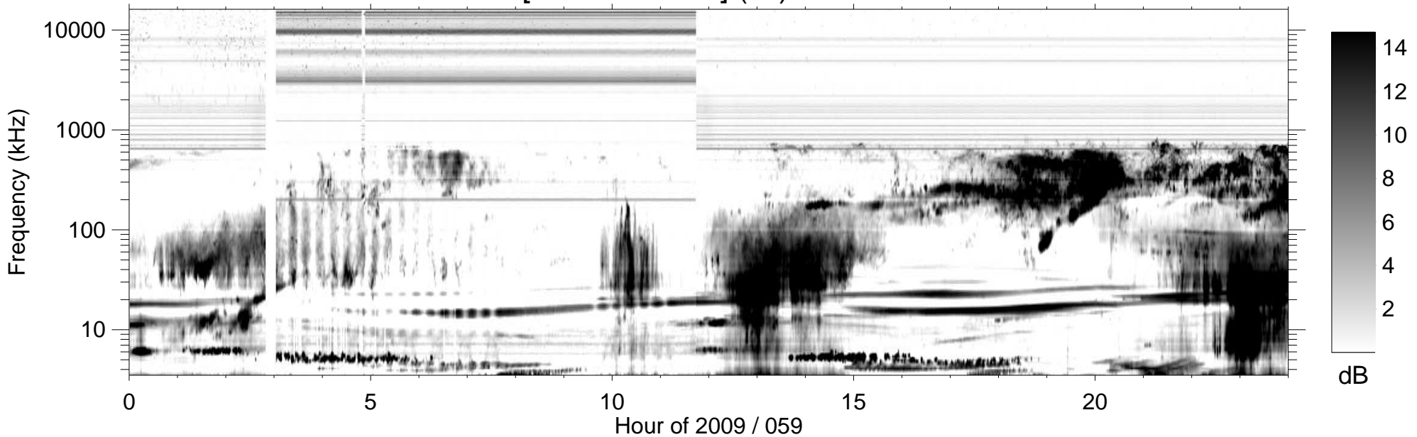
RPWS [ABCH1H2/Ex] (-B) 2009/02/28
