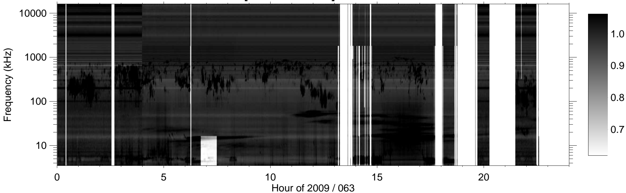
RPWS [ABCH1H2/Ex] (-B) 2009/03/04
