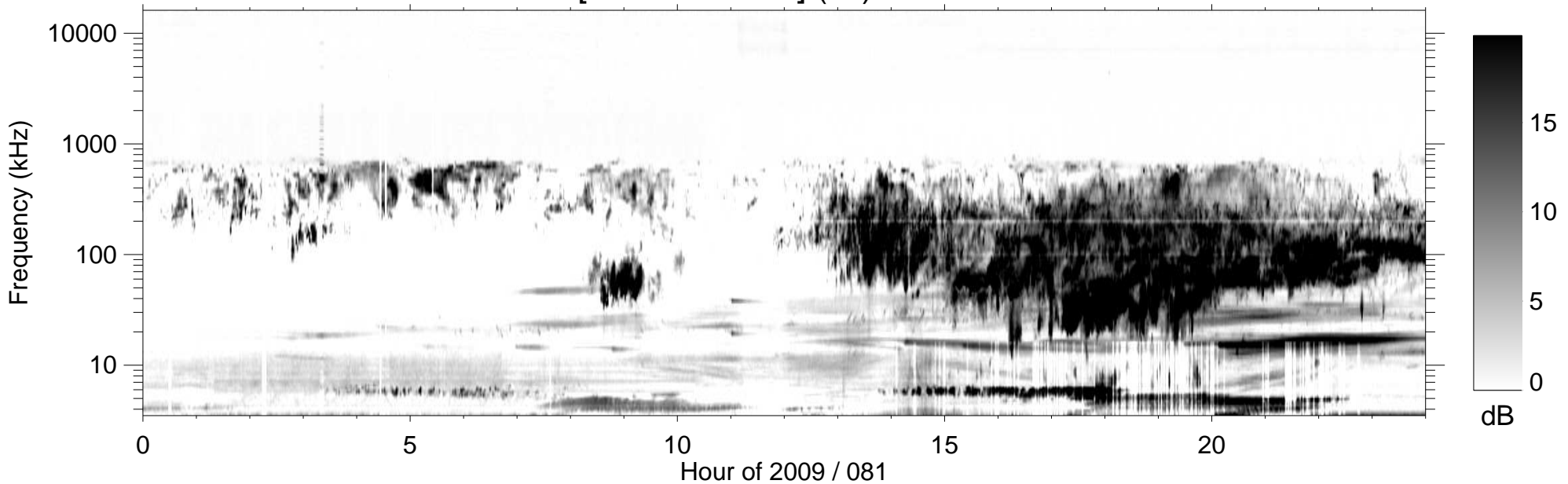
RPWS [ABCH1H2/Ex] (-B) 2009/03/22
