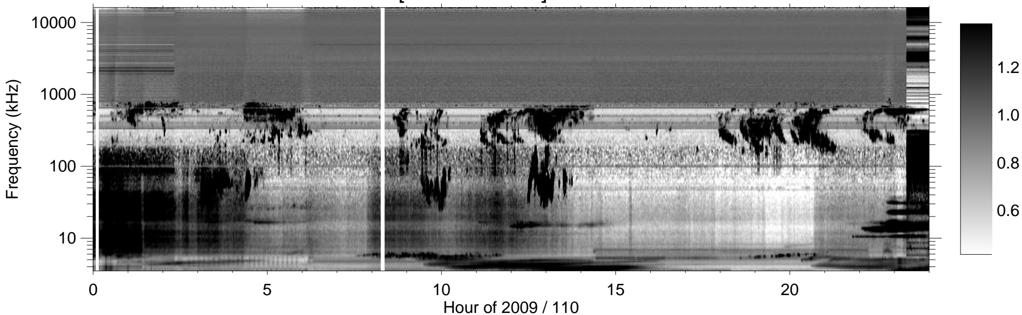
RPWS [ABCH1H2/Ex] (-B) 2009/04/20
