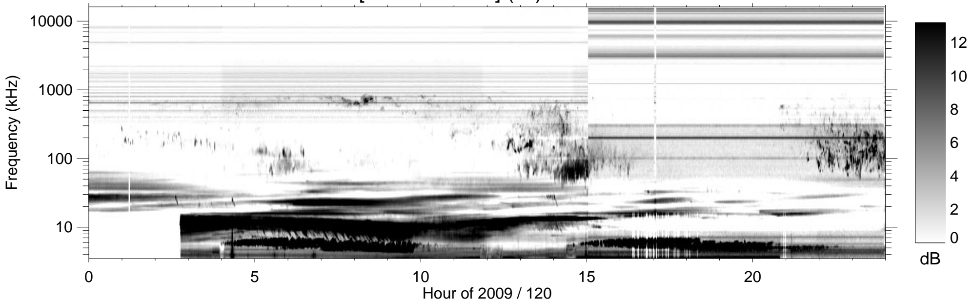
RPWS [ABCH1H2/Ex] (-B) 2009/04/30
