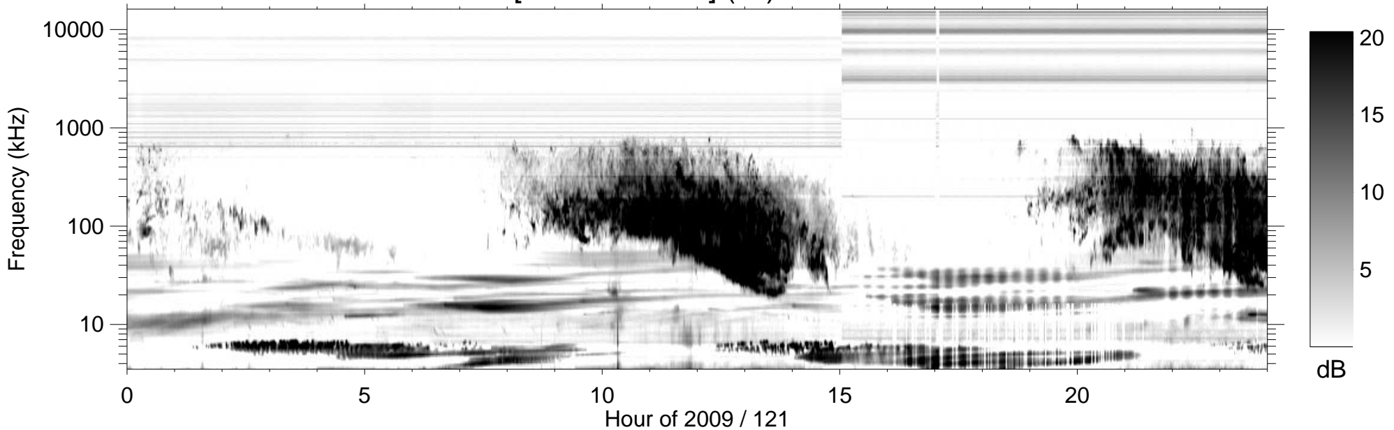
RPWS [ABCH1H2/Ex] (-B) 2009/05/01
