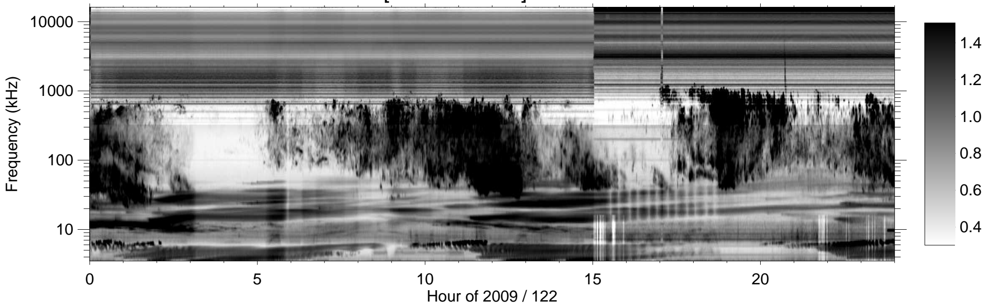
RPWS [ABCH1H2/Ex] (-B) 2009/05/02
