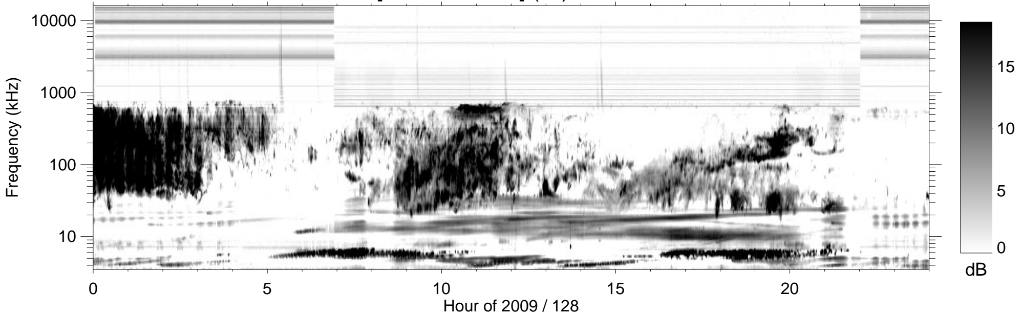
RPWS [ABCH1H2/Ex] (-B) 2009/05/08
