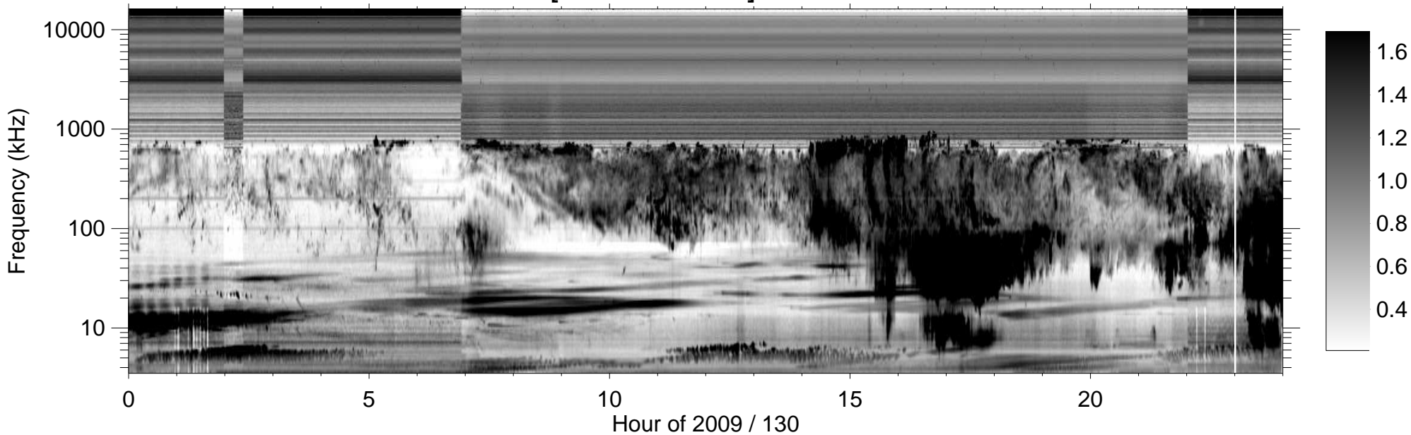
RPWS [ABCH1H2/Ex] (-B) 2009/05/10
