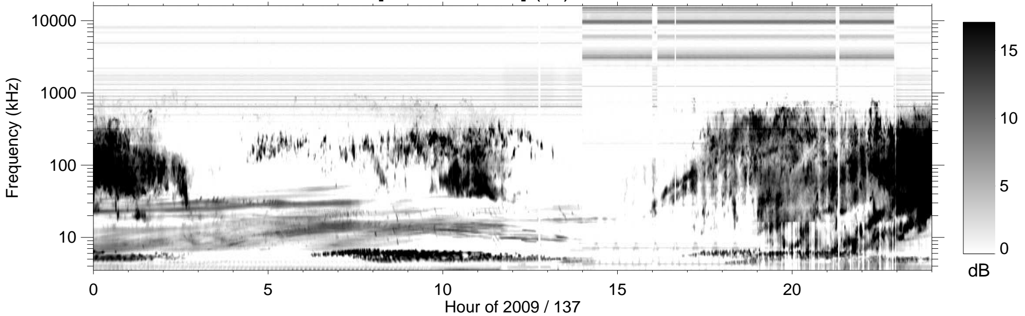
RPWS [ABCH1H2/Ex] (-B) 2009/05/17
