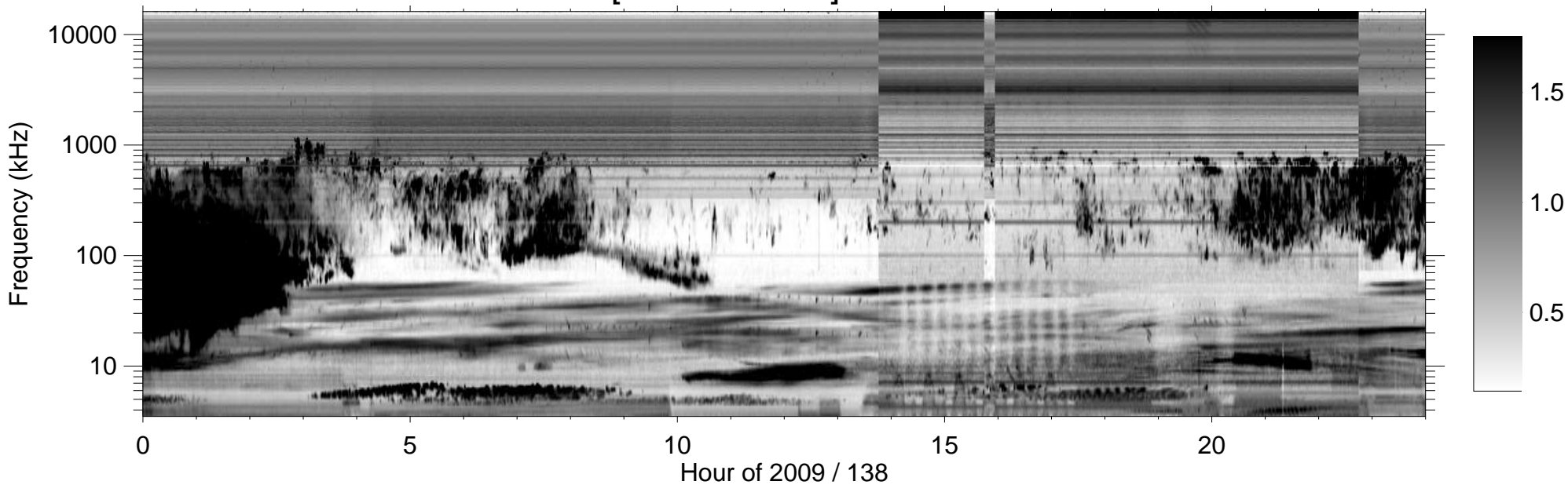
RPWS [ABCH1H2/Ex] (-B) 2009/05/18
