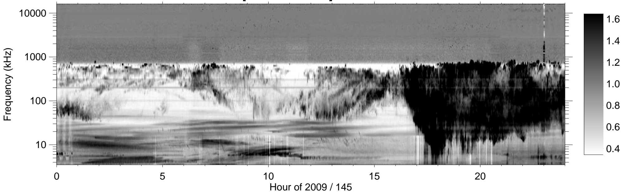
RPWS [ABCH1H2/Ex] (-B) 2009/05/25
