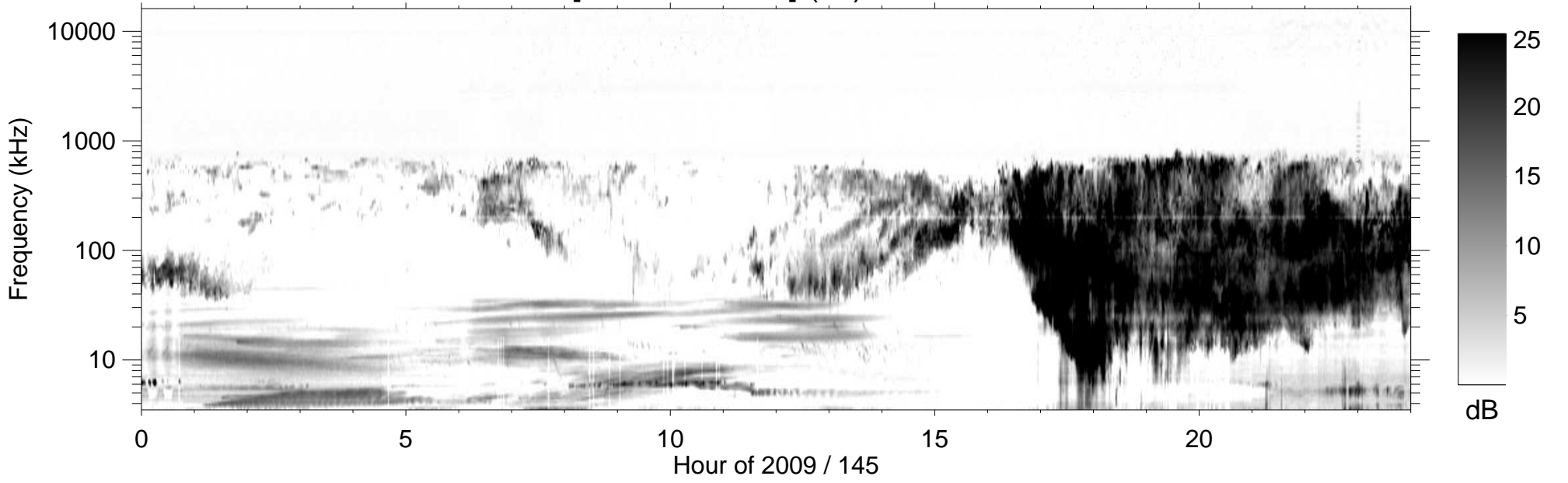
RPWS [ABCH1H2/Ex] (-B) 2009/05/25
