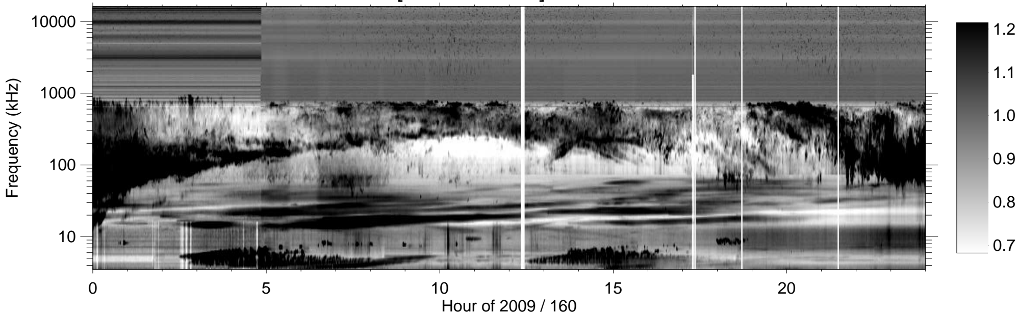
RPWS [ABCH1H2/Ex] (-B) 2009/06/09
