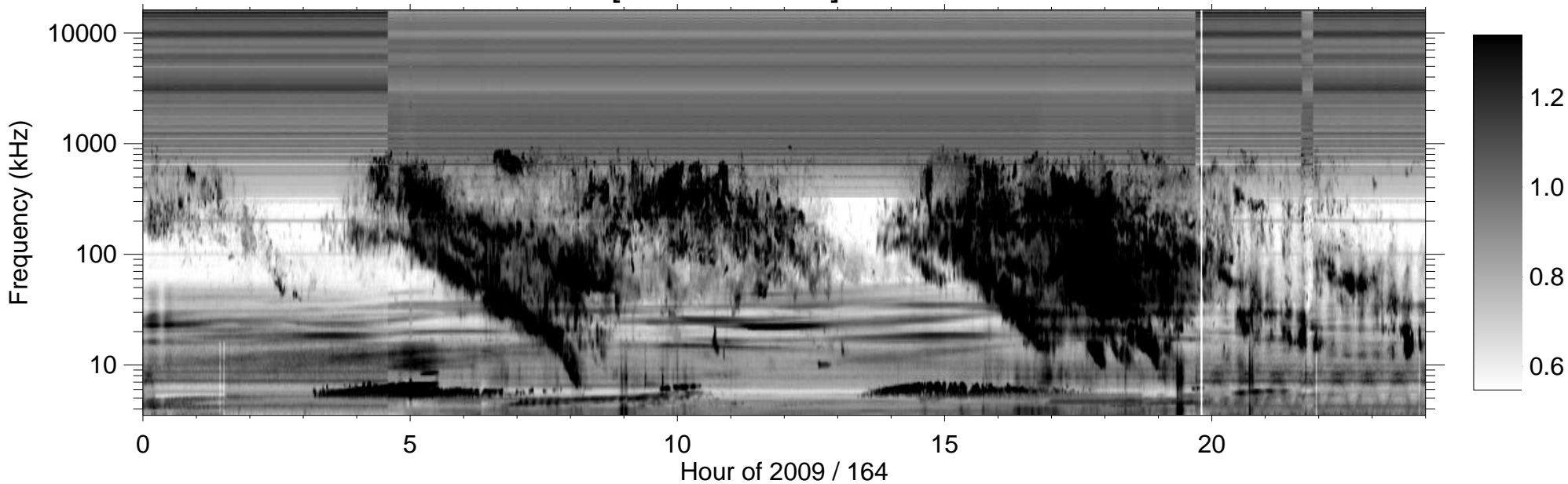
RPWS [ABCH1H2/Ex] (-B) 2009/06/13
