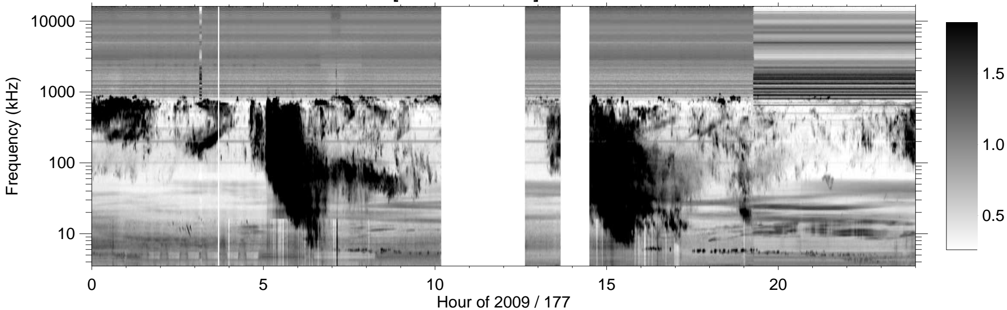
RPWS [ABCH1H2/Ex] (-B) 2009/06/26
