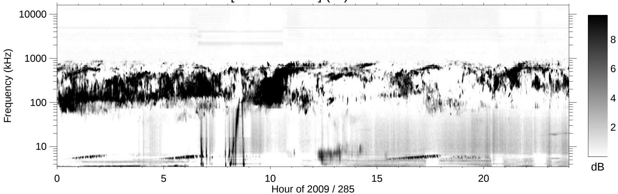
RPWS [ABCH1H2/Ex] (-B) 2009/10/12
