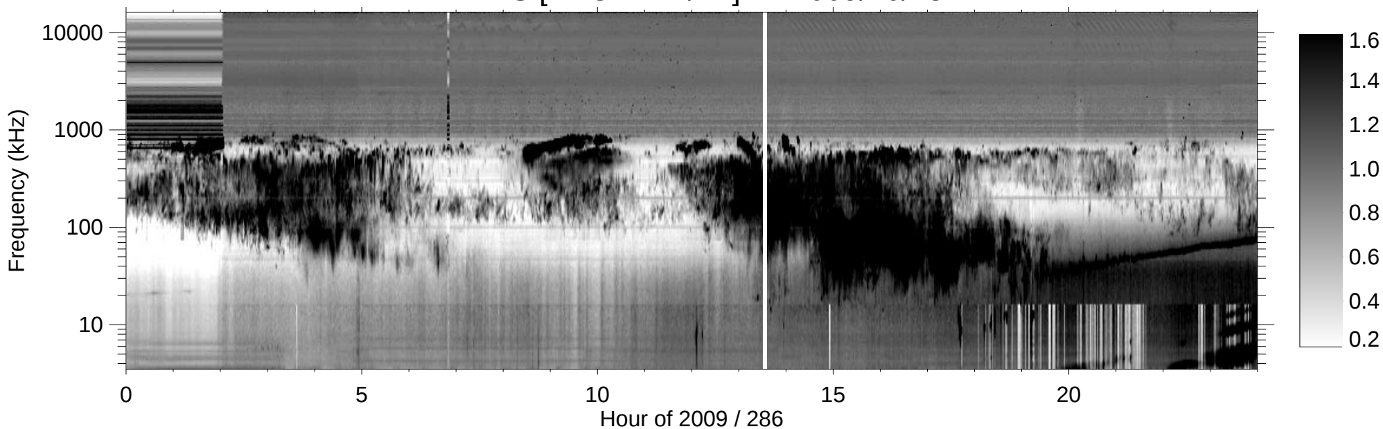
RPWS [ABCH1H2/Ex] (-B) 2009/10/13
