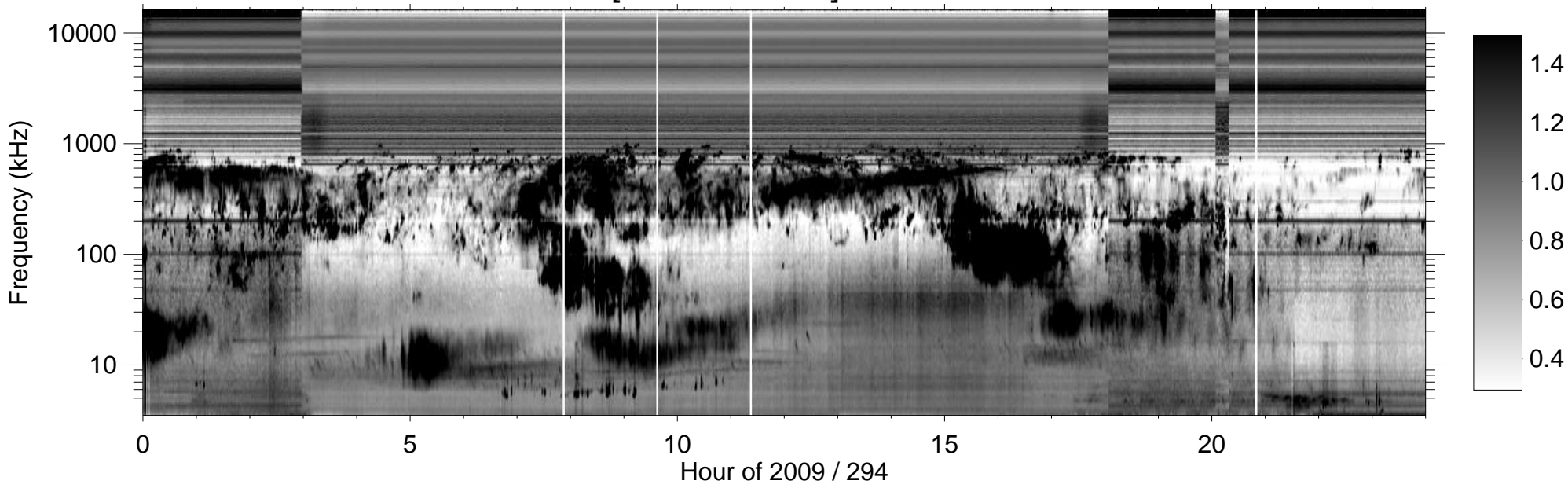
RPWS [ABCH1H2/Ex] (-B) 2009/10/21
