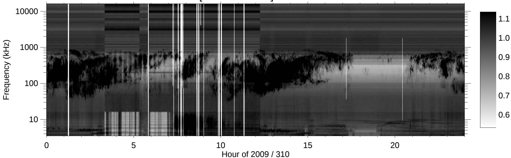
RPWS [ABCH1H2/Ex] (-B) 2009/11/06
