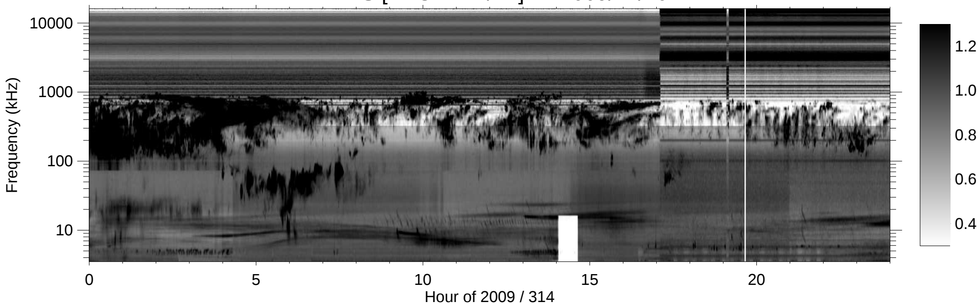
RPWS [ABCH1H2/Ex] (-B) 2009/11/10
