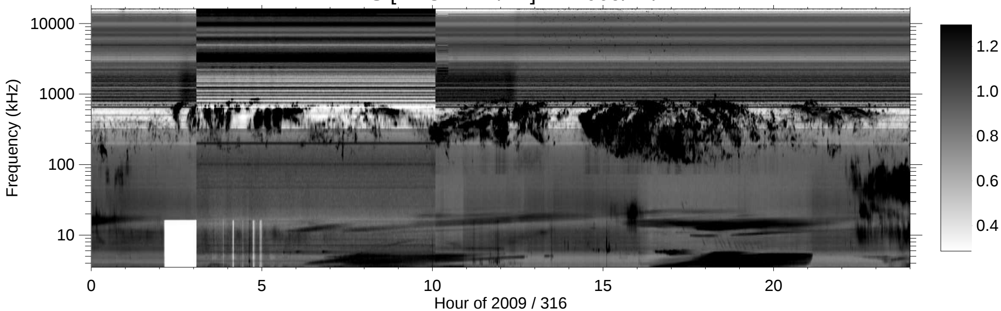
RPWS [ABCH1H2/Ex] (-B) 2009/11/12
