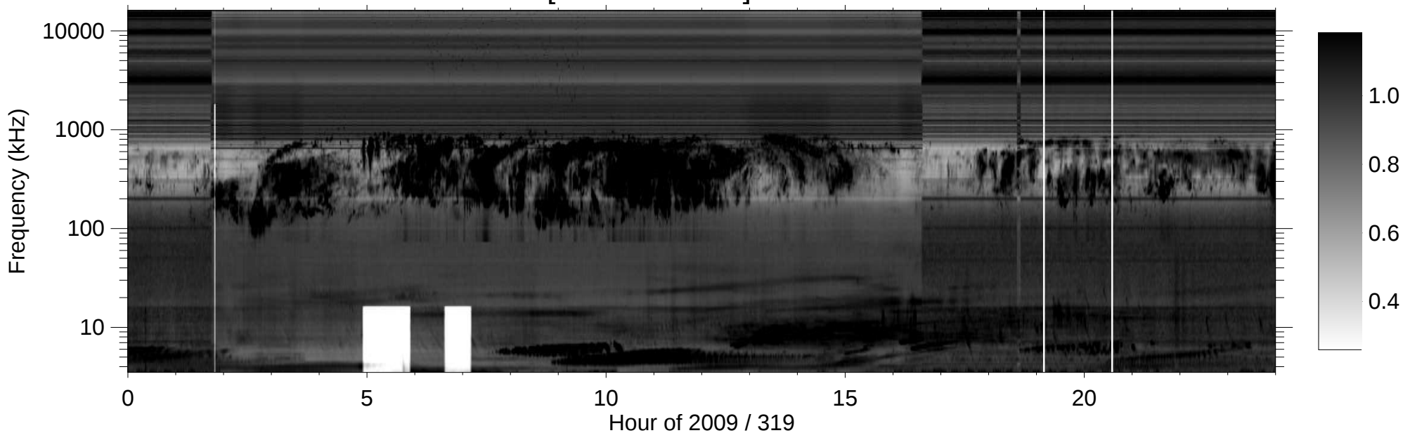
RPWS [ABCH1H2/Ex] (-B) 2009/11/15
