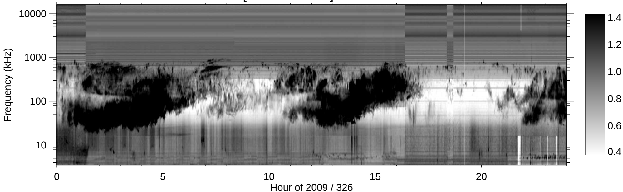
RPWS [ABCH1H2/Ex] (-B) 2009/11/22
