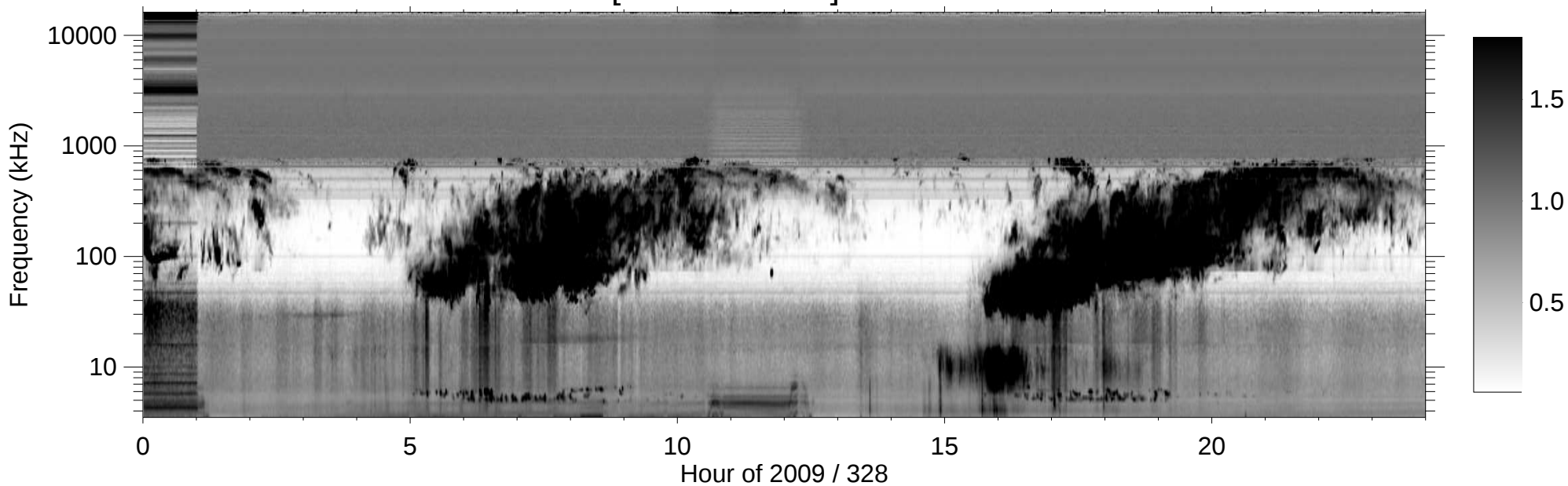
RPWS [ABCH1H2/Ex] (-B) 2009/11/24
